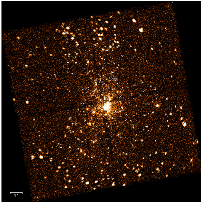
Orion from space
